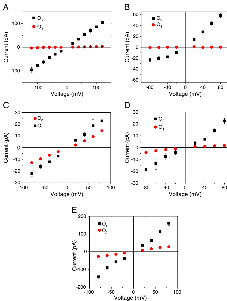
Fig. 4. Current–voltage (I–V) profiles of all sub-states of the members of the OccD subfamily. (A) OccD1; (B) OccD3; (C) OccD4; (D) OccD5 and (E) OccD6. The data shown in these panels represent the average of at least three independent experiments. The lack of some data points is due to the low frequency and/or amplitude of these flickering events at a low applied transmembrane potential. OccD2 data is not shown owing to the large variability in the baseline of O_1 and O_2 open sub-states. The buffer solution was 1 M KCl, 10 mM potassium phosphate, pH 7.4.
