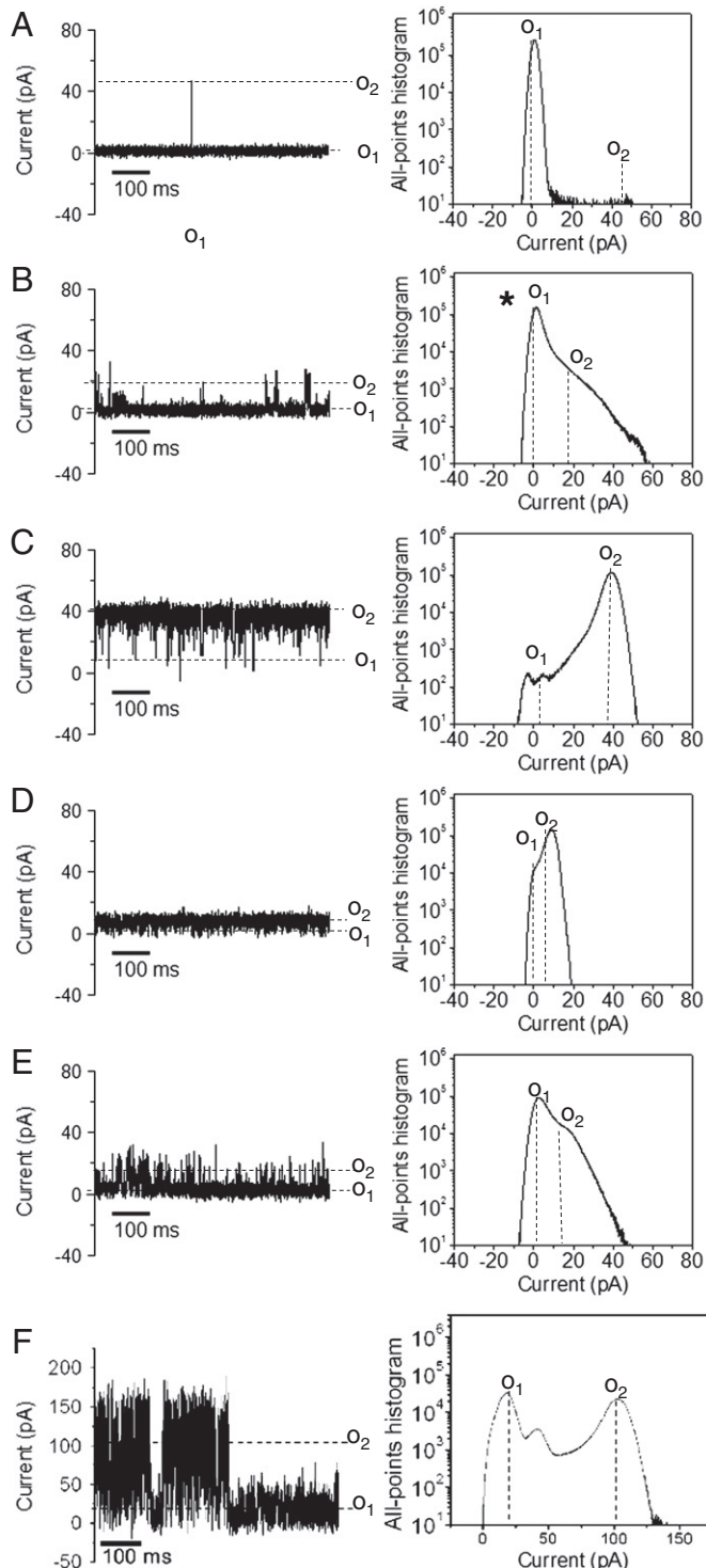
Fig. 2. Typical single-channel electrical traces of six members of the OccD subfamily and their corresponding all-points current amplitude histograms. The single-channel electrical traces were recorded at a transmembrane potential of +60 mV. The buffer solution was 1 M KCl, 10 mM potassium phosphate, pH 7.4. (A) OccD1, (B) OccD2, (C) OccD3, (D) OccD4, (E) OccD5 and (F) OccD6. Current levels were marked both on the single-channel electrical traces and on the all-points current amplitude histograms. All single-channel electrical traces were low-pass Bessel filtered at 2 kHz. The "*" is indicated for the OccD2 channel, whose baseline of the O_1 open sub-state varied between 2 and 17 pA. All electrical traces were representative over at least three independent single-channel electrical recordings.
