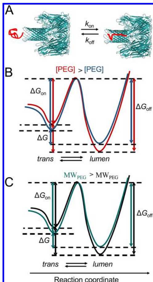
Figure 6. Free energy profile of the Syn B2– \alpha HL interactions. (A) Cartoon showing the two substates of the Syn B2 polypeptides, in the trans conformation (“ trans ”) and under nanopore confinement (“ lumen ”). (B) Qualitative representation of the free energy profile at an increased concentration of less-penetrating PEGs. (C) Qualitative representation of the free energy profile at an increased PEG molecular size.
